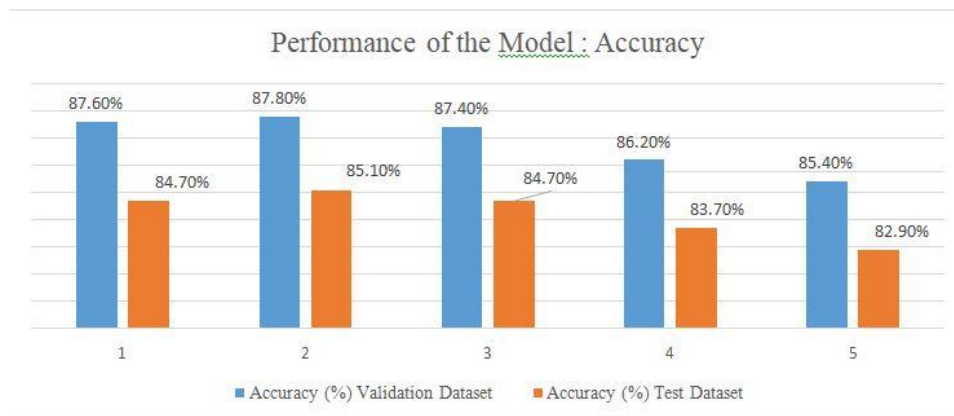
Figure 4. The accuracy of the classifiers for diabetic prediction based on validation and test dataset
