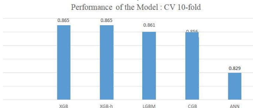
Figure 10. The MCC of the classifiers for diabetic prediction based on validation and test dataset ...
