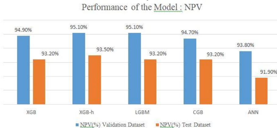
Figure 9. The NPV of the classifiers for diabetic prediction based on validation and test dataset ...
